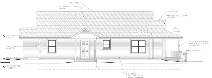
SIDE BUILDING ELEVATION
