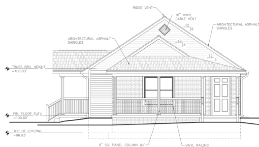
FRONT BUILDING ELEVATION
